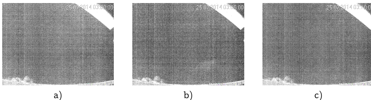
Figure 1. Local glow visible from Hasanya, corresponding to the maximum period (03:05) of the local eastern electric jet: a) 03:00, b) 3:05 LT, c) 03:10. The photo was taken with a Cs265 camcorder, used in black and white resolution in the "night" mode. Brightness increased 15 times
